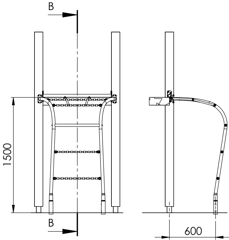
SECTION B-B
